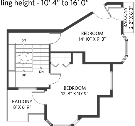
Level 3 - 613 sq.ft. Ceiling height - 10' 4" to 16' 0"
